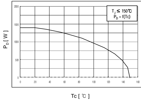
Fig 10. Power Dissipation vs. Case Temperature
