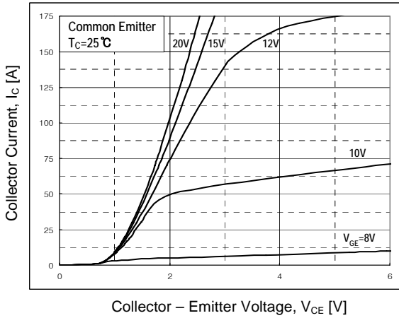
Collector - Emitter Voltage, V_{CE} [V] Fig 1. Typical Output characteristics
