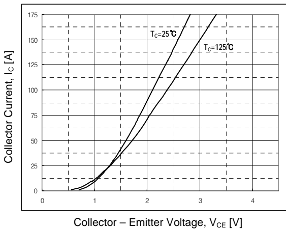
Collector - Emitter Voltage, V_{CE} [V] Fig 3. Typical Saturation Voltage characteristics
