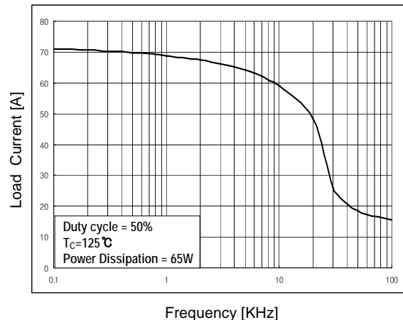
Frequency [KHz] Fig 4. Load Current vs. Frequency
