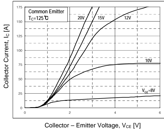
Collector - Emitter Voltage, V_{CE} [V] Fig 2. Typical Output characteristics
